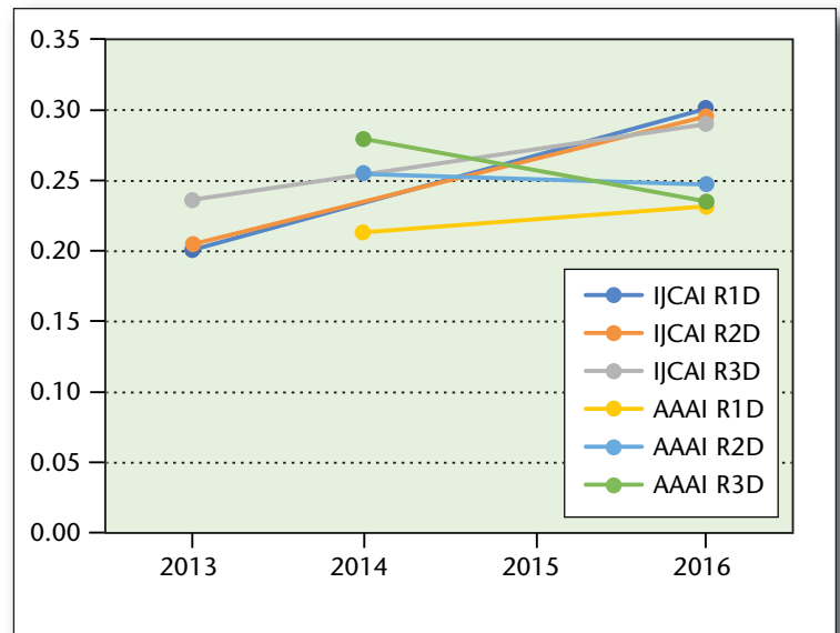
Figure 3. Change Over Time of the Three Reproducibility Metrics for Selected Years of the Two Conferences AAAI and IJCAI.
