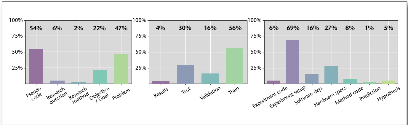
Figure 1. Percentage of Papers Documenting Each Variable for the Three Factors Method (left), data (middle), and experiment (right). Gundersen and Kjensmo (2018).
