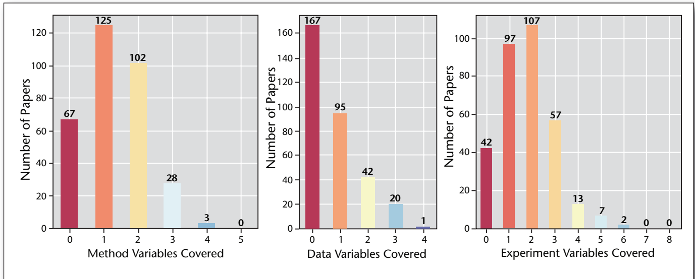
Figure 2. The Number of Variables for the Three Factors as Documented for All the Papers Describing Empirical Research in the Study. Method (left), data (middle), and experiment (right). Gundersen and Kjensmo (2018).
