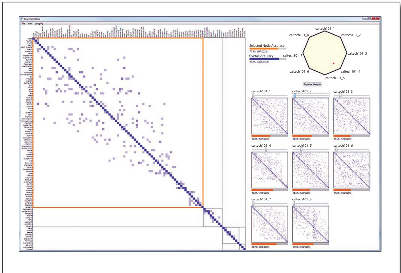
Figure 8. EnsembleMatrix.
