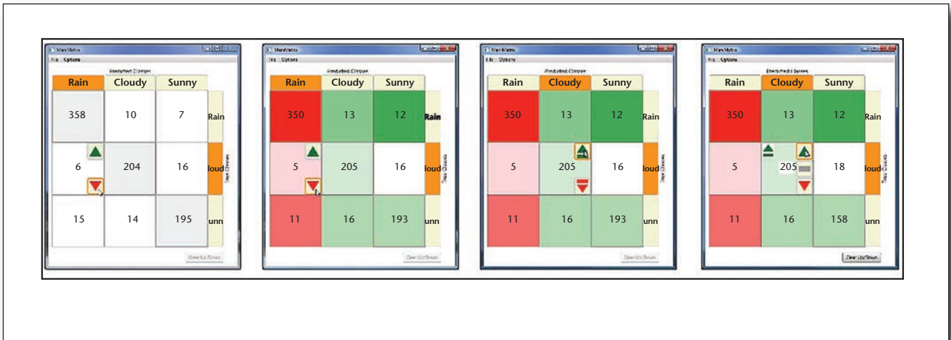
Figure 7. ManiMatrix System.
