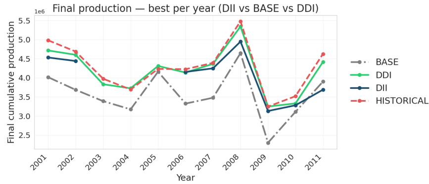
Figure 3: Comparison of final dry-season cumulative production (MWh) for the Minimum-release baseline (BASE), DDI, DII, and Historical operations.
