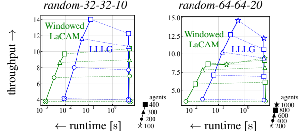
Figure 9: Effect of anytime improvement on the algorithms. The planning runtime budget is 5 s/step in both maps. Dashed lines connect each algorithm to its anytime variant.
