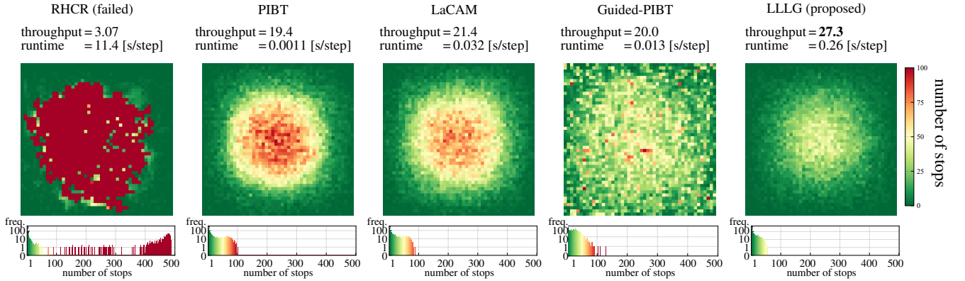
Figure 3: Heatmap of vertex stop counts, where congestion is implied by warm colors. The bottom of each heatmap shows the distribution among vertices of how many times each vertex is used as a stop by any agent.
