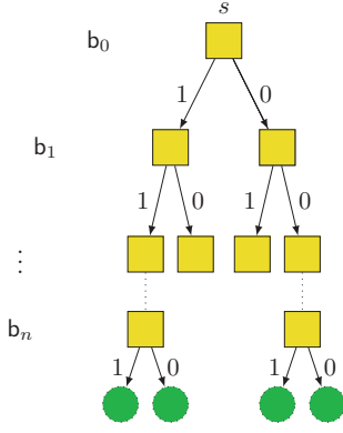
Figure 2: Example for a factored decision node tree. Each layer corresponds to the assignment of a single base action.
