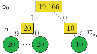
Figure 3: Search tree of a multi-armed bandit problem based on factored representation.
