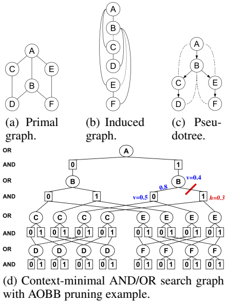
Figure 1: Example problem with six variables, induced graph along ordering A, B, C, D, E, F , corresponding pseudotree, and resulting AND/OR search graph with AOB pruning example.
