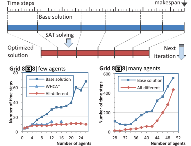
Figure 2. Illustration of the optimization process and makespan comparison on the 8 \times 8 grid. Optimal solutions for up to 22 can be found. Only up to 16 agents can be solved by WHCA*.
