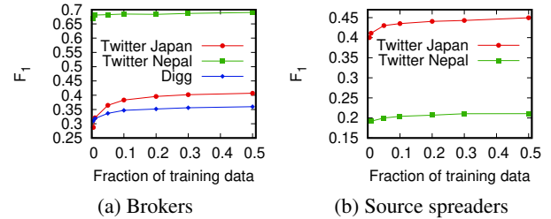
Figure 4: Effects of amount of training data when predicting top-10% influencers. Using 5% training data achieves F_1 scores that are similar to those with 50% training data.
