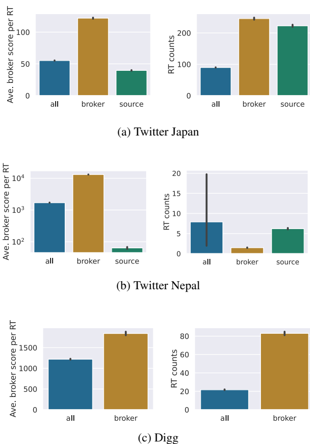
Figure 3: Comparison of average broker score per retweet and the number of retweets posted by users among influential source spreaders, influential brokers, and all users. A tweet retweeted by an influential broker tends to spread more widely than does a tweet retweeted by an influential source spreader.
