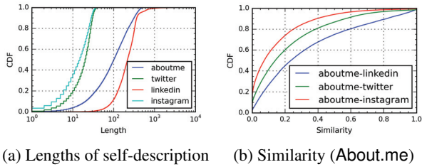
Figure 2: Difference of self-descriptions: (a) Distribution of lengths of self-description and (b) pair-wise TF-IDF similarity scores across different social networks.
