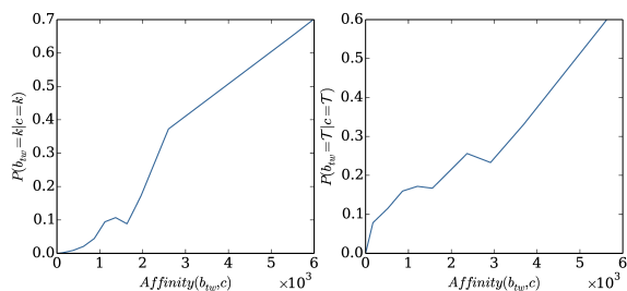
Figure 6: Influence of Twitter-based Kickstarter communities over the backing habits of users.
