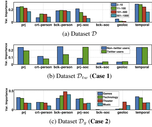
Figure 8: Variable importance of various Kickstarter features. (a)-(c) shows the AUC value improvements over 0.5 when using only a particular feature set.
