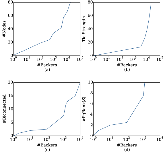
Figure 4: Impact of Twitter network on the backers of Kickstarter projects. (a) shows the impact of a promoter count, (b) and (c) shows the importance of connectivity in the network of promoters, and (d) shows the importance of influential promoters.
