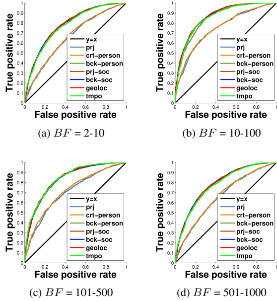
Figure 7: The ROC curve results for different backing frequency ( BF ) values.
