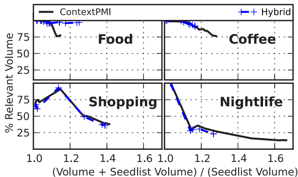
Figure 3: Quality vs. quantity in identified tweets. Each point corresponds to the inclusion of 10 additional keywords.
