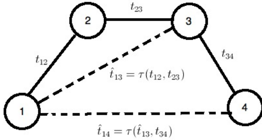
Figure 1: Trust propagation.
