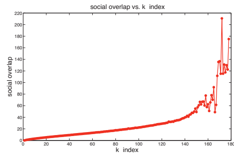
(b) Average social overlap vs k -index
