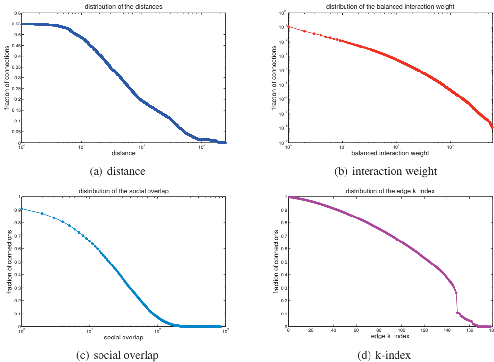
Figure 2: Complementary cumulative distribution function of spatial length, balanced interaction weight, social overlap and k -index for the social ties in the Tuenti social network.
