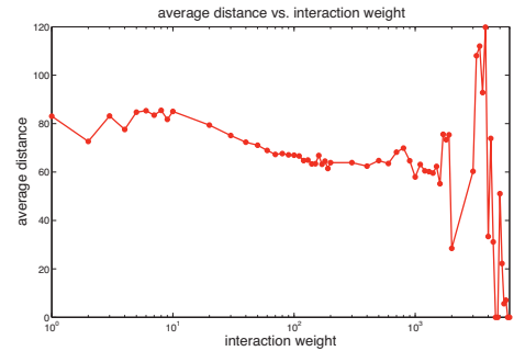
Figure 8: Average link length as a function of interaction weight.
