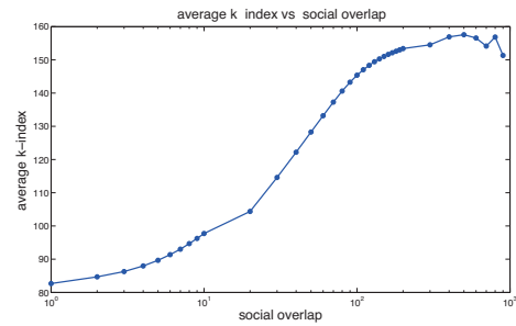
(a) Average k -index vs social overlap
