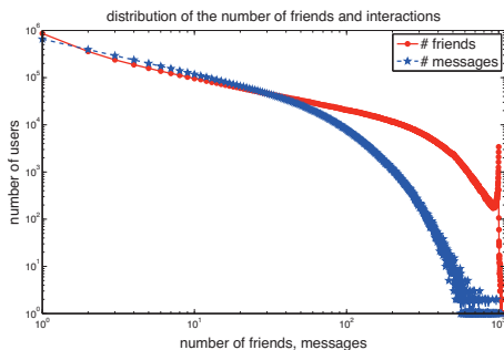
Figure 1: Complementary cumulative distribution of the number of friends and messages sent by Tuenti users.
