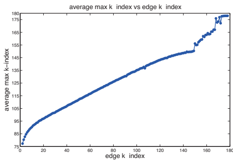
Figure 4: Average value of the maximum k -index of the two endpoints of an edge as a function of edge k -index.
