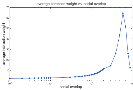
(a) Average social overlap vs interaction weight
