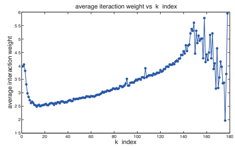
(a) Average k -index vs interaction weight
