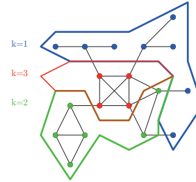
Figure 3: An example of the k -core decomposition.
