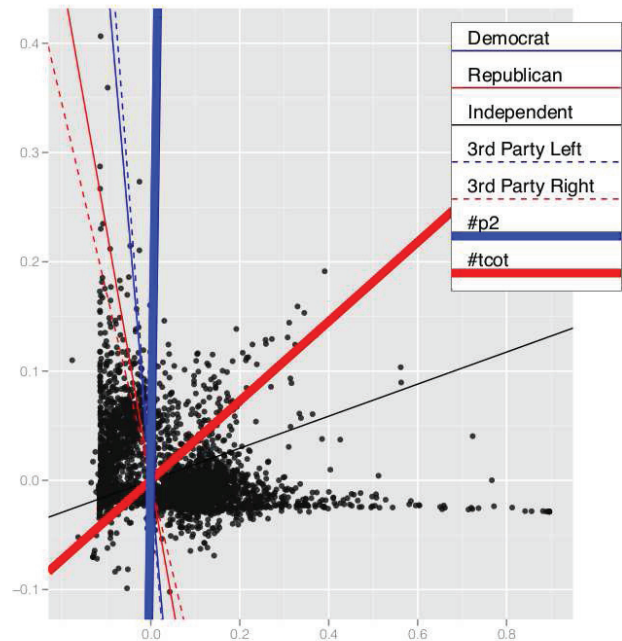
Figure 1: Multidimensional scaling with trend lines. Stress: 2.55
