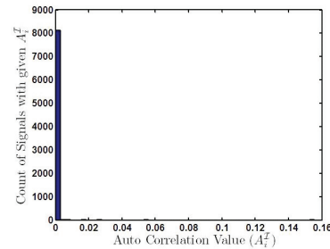
Figure 3: Skewed Distribution of Auto Correlation Values \theta_1 , EDCoW first computes the median absolute deviation ( MAD ) of all A_i^{\mathcal{I}} within \mathcal{S}^{\mathcal{I}} :
