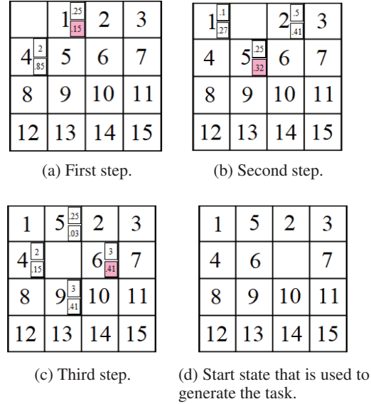
Figure 2: Hypothetical simulation of GenerateTask after training on the task that was generated with start state as in figure 1c.
