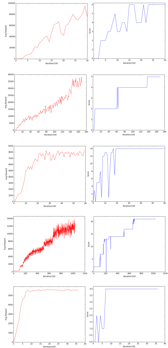
Figure 3: Average reward and scores over number of iterations. Row 1: Breakout MOVE + FIRE 4x6 bricks (5 minutes); Row 2: Breakout MOVE only 4x5 bricks (1 hour); Row 3: Sapientino S2 OMNI (3 minutes); Row 4: Sapientino S3 DIFFERENTIAL (1 hour); Row 5: Cocktail Party (3 minutes).
