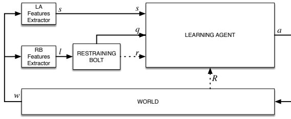
Figure 1: Learning Agent and Restraining Bolt
