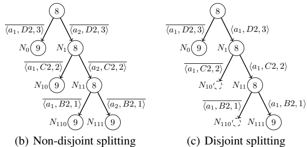
Figure 1: (a) A 2-agent MAPF instance on a 4-neighbor grid. (b) and (c) The corresponding CT of CBS with non-disjoint splitting and with disjoint splitting, respectively. Solid nodes are labeled with their costs, and edges are labeled with the constraints they enforce. Dashed nodes are pruned.
