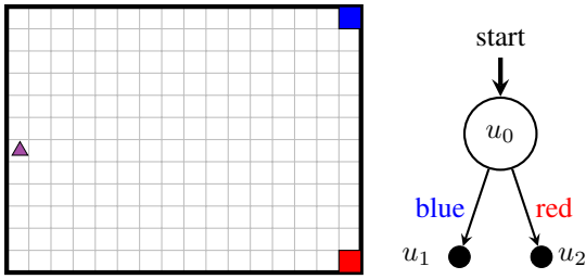
Figure 4: Double Slit environment (left) and FSA task specification to reach either goal locations blue or red.
