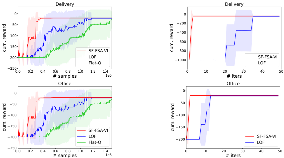
Figure 3: Experimental results for learning (Delivery, top-left and Office, bottom-left) and compositionality (Delivery, top-right and Office, bottom-right). Results show the average performance and standard deviation over the three tasks and 5 seeds per task.
