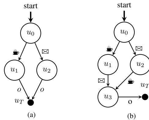
Figure 2: Disjunction (a) and composite (b) FSA task specifications for the Office domain.
