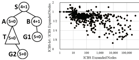
Figure 4: ICBS versus ICBS- h .
