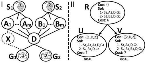
Figure 1: (I) A MAPF instance. (II) Its CT.
