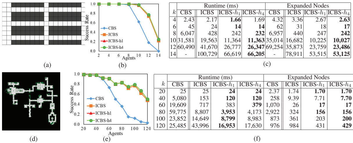
Figure 3: Experimental results on a warehouse grid (top) and a computer game grid (bottom).
