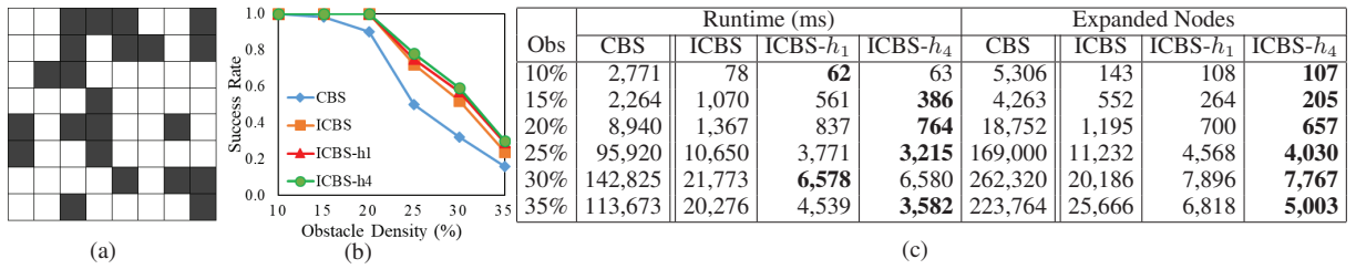
Figure 2: Experimental results on 8 \times 8 grids.
