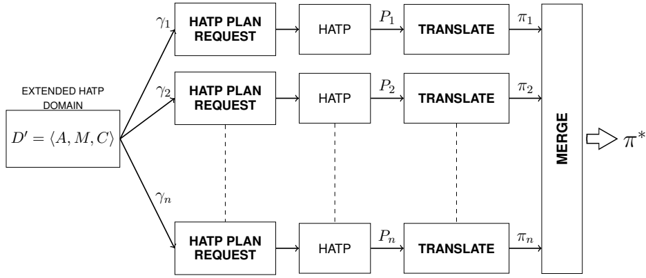
Figure 1: Architectural schema of the proposed system.
