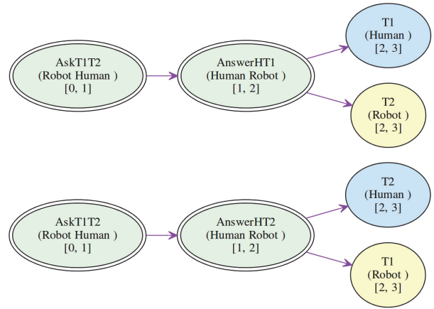
Figure 2: HATP plans for HumanChoosesT1 and HumanChoosesT2 .
