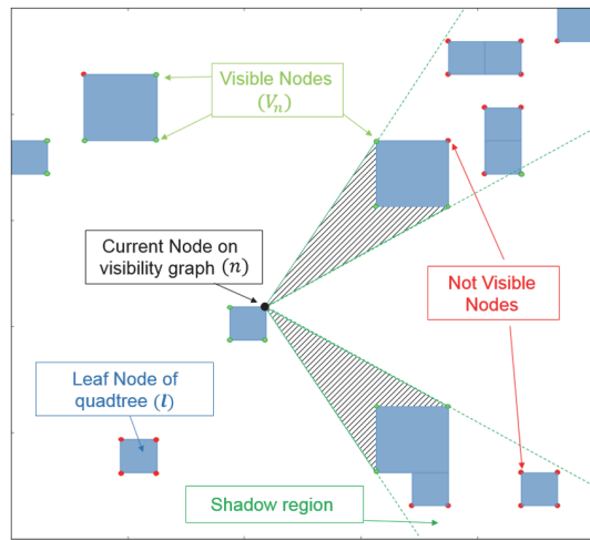
Figure 3: Computation of visible nodes in quadtree.
