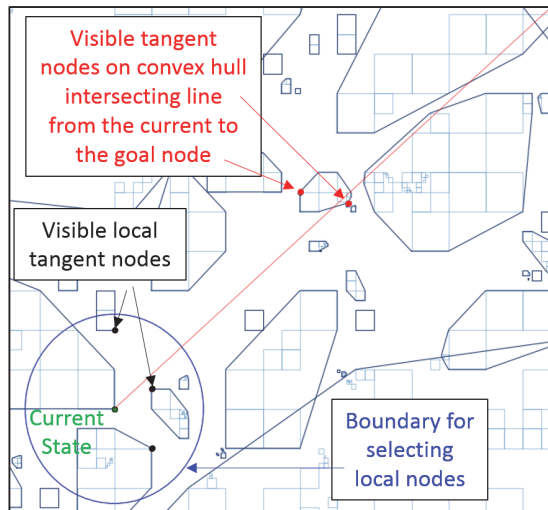
Figure 9: Procedure to add nodes to the focused visibility graph.
