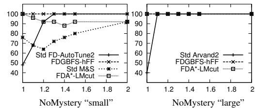
Figure 5: % instances covered in Nakhost et al.’s (2012) NoMystery test suites, over resource constrainedness (factor by which the available fuel exceeds the minimum required).
