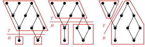
Figure 1: Examples of “horizontal lines” \{T, B\} through a DAG of SCCs, and the corresponding fork factorings.
