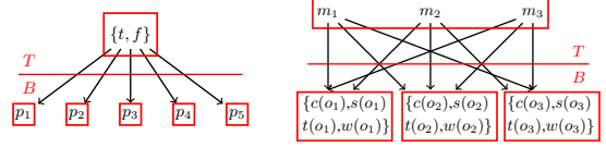
Figure 2: Possible fork factorings in transportation with fuel consumption (left), and job-planning problems (right).
