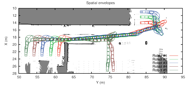
Figure 8: Spatial envelopes generated for a set of vehicles in a logistics environment.
