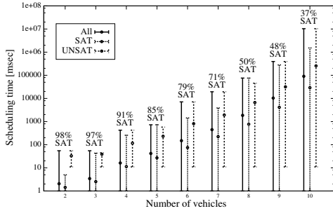
Figure 6: Quantitative evaluation of the coordinator.
