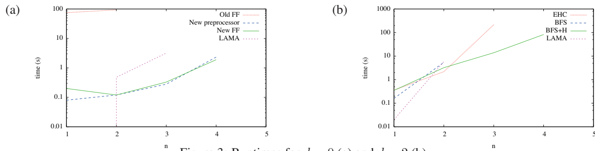
Figure 3: Runtimes for d = 0 (a) and d = 2 (b).
