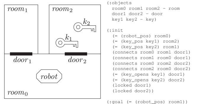
Figure 1: Unsolvable task in the Keys domain with corresponding PDDL code.
