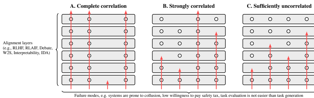
Figure 1: Correlation of failure modes governs defense-in-depth. A: Fully correlated presence/absence across layers (here, modes 1, 2, 4 succeed; mode 3 is universally absent and blocks at entry). B: Strong correlation leaves one shared mode (one straight-through attack), while others are blocked early. C: Sufficiently uncorrelated modes each block the attack at different layers.
