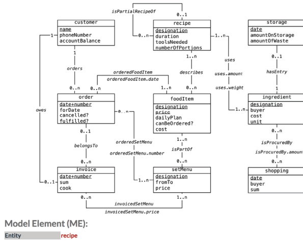
Figure 2: Model verification task containing (a) the evidence scenario, the EER model and model element and (b) questions for guiding the verification process.
