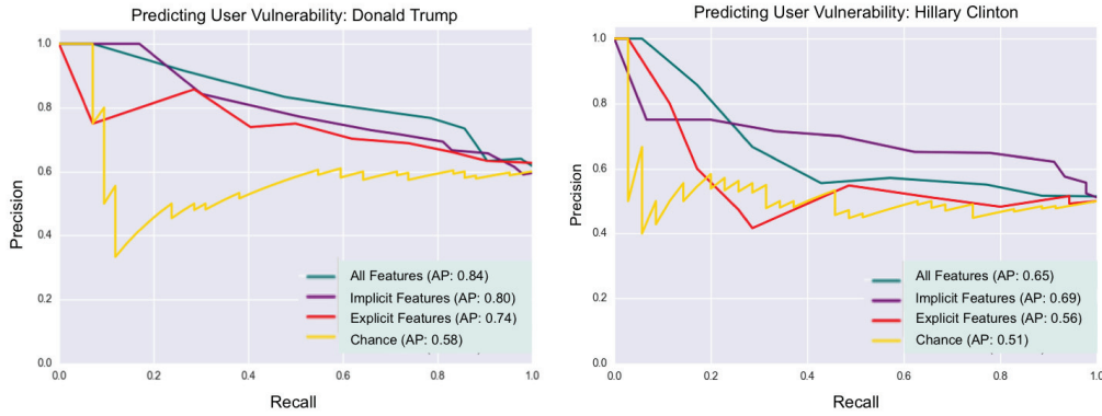
Figure 3: Shown are precision-recall curves and average precision (AP) scores for all prediction systems; Trump (left), Clinton (right). Our Crowd-O-Meter system (i.e., All Features ) outperforms today’s status quo approach (i.e., Chance predictions) by up to 26 percentage points (i.e., Trump), showing the promise of our proposed novel task to model human vulnerability. Our results also highlight that a user’s unconscious behavioral data (purple curve) is a better predictor than relying on a user’s explicitly shared information (red curve) alone.
