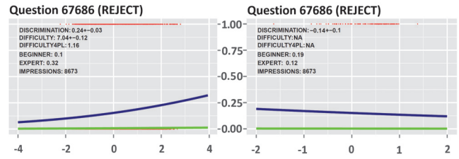
Figure 8: Example of rejected Production Question based on endogenous (left) vs. exogenous (right) metrics. The X-axis is the test-taker ability \theta and the Y-axis is the probability P(\theta) of answering the question correctly (blue curve) and I(\theta) is the Fisher information (green curve).
