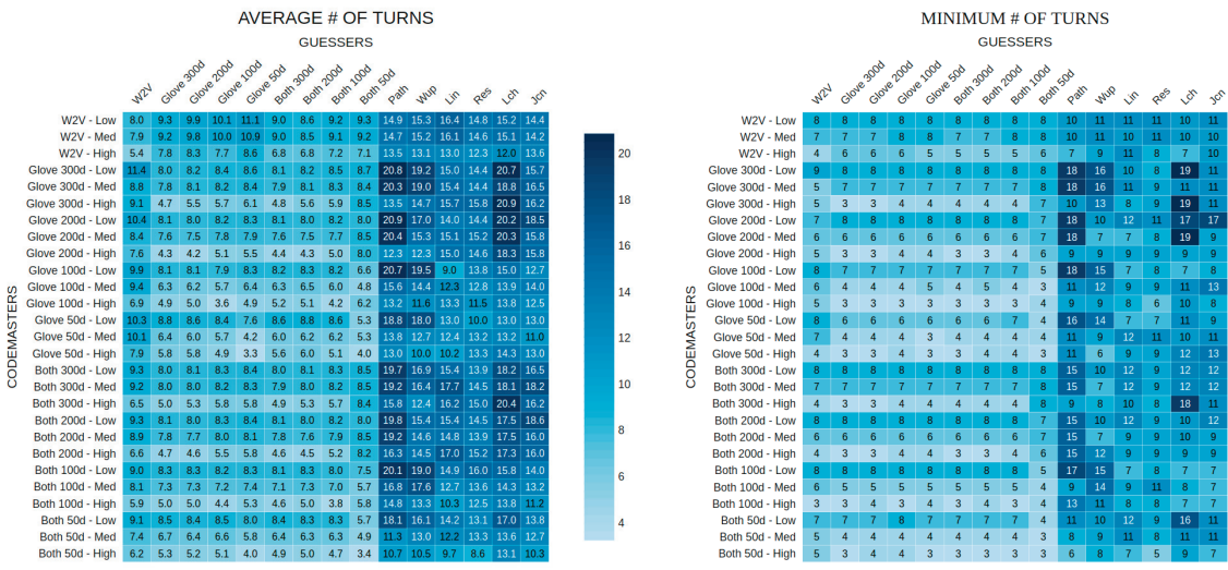
Figure 1: The average (left) and minimum (right) number of turns that the different pairs take to finish the game. These turn counts are based only on games that are won, ignoring the games where the team loses. Lighter cells are better than darker. We see that the more aggressive thresholds lead to better min and average turn counts – with 3 turn wins not being uncommon. The more conservative thresholds lead to 7 or 8 turn games – 1 clue per turn. We notice that while the various vectorial semantic approaches work well together, the WordNet based approaches universally do not play well with vectorial semantic approaches.
