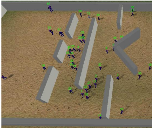
Figure 2: Successfully navigating a maze . The agents spawn from the left side of the maze and proceed to an enemy at the right. They learn to navigate mazes through gradual training on increasingly difficult wall configurations.
