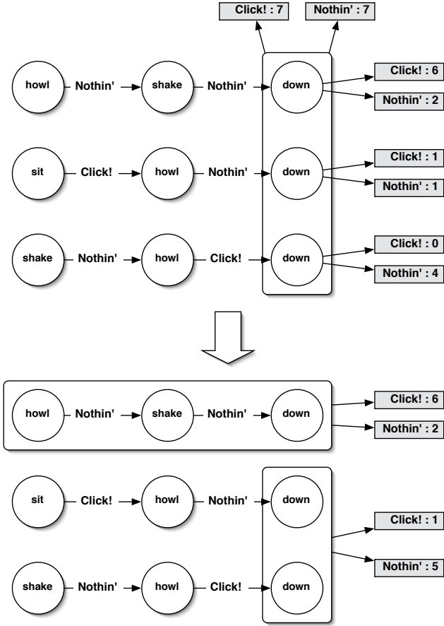
Figure 2: OFESI action splitting method for synthetic characters
