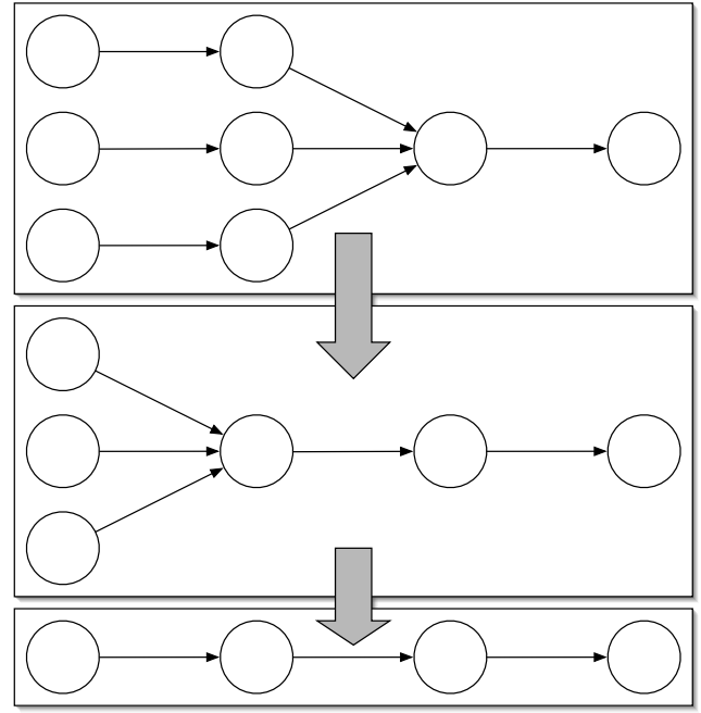
Figure 3: Learning long action chains, first proposal
