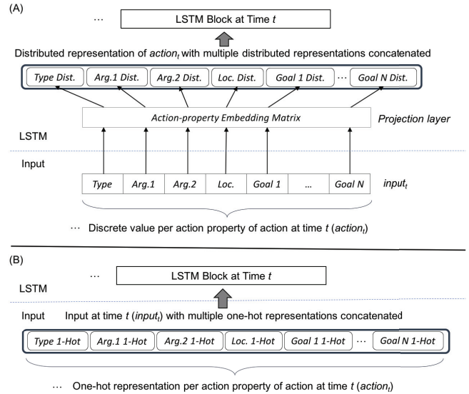
Figure 4: (A) LSTM incorporating a projection layer to learn distributed representations of actions (Min et al. 2016a). The number of input features for a single action is N+4 , (B) LSTM with one-hot encoded action inputs. The number of input features is 227+13*N , where 13 is derived from 12 possible goals plus “None”, and 227 are the total number of possible values for the other action properties. In both figures, N is the number of previously achieved goals to be considered by the models. In this work, it is set to 12.
