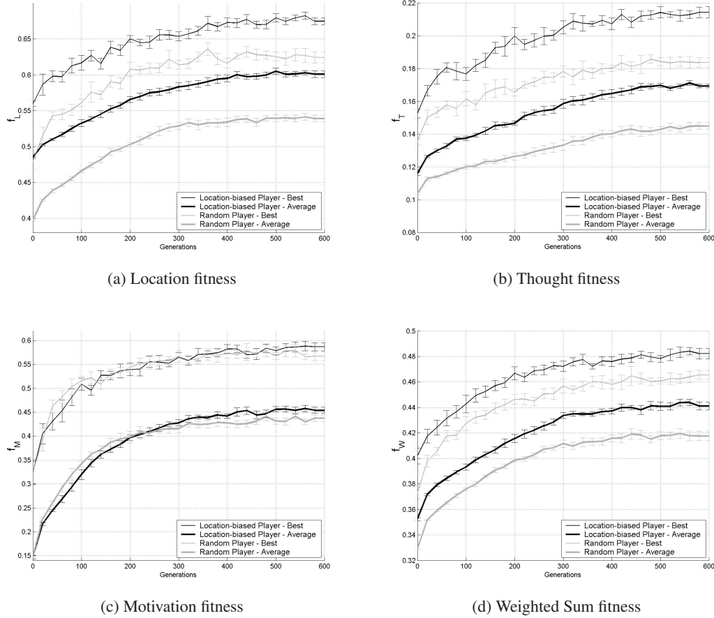
Figure 3: Evolution of the fitness functions tested across the two player models (Location-biased and Random). Figures depict average values of 10 runs and corresponding 95% confidence interval bars every 20 generations.
