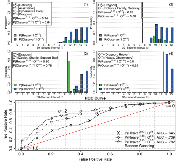
Figure 3: Top (Barplots): the prediction results for Query A applied to Reaver and Observer units for a single game. Bottom: the ROC curve for the Reaver-prediction task over all games (5-fold cross validation).
