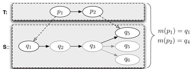
Figure 3: A phase mapping between target T and source S .
