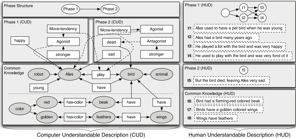
Figure 1: Complete representation of a basic story.
