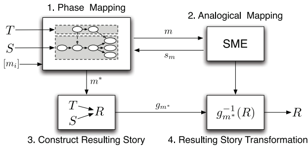
Figure 2: The four steps of the SAM algorithm.
