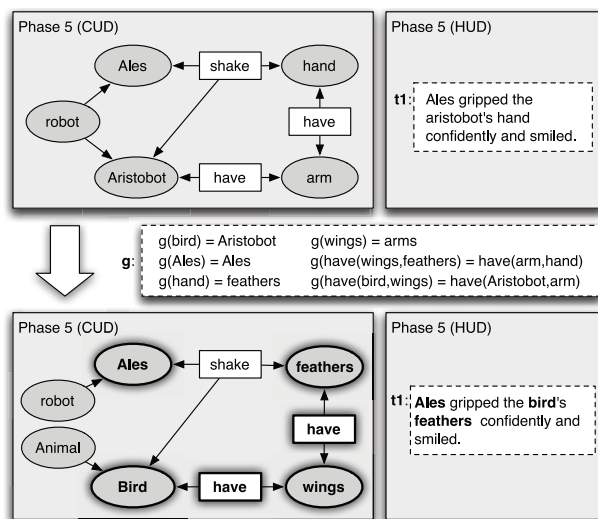
Figure 4: Transformation of a phase in the resulting story by reversing the analogical mapping g found by SME.
