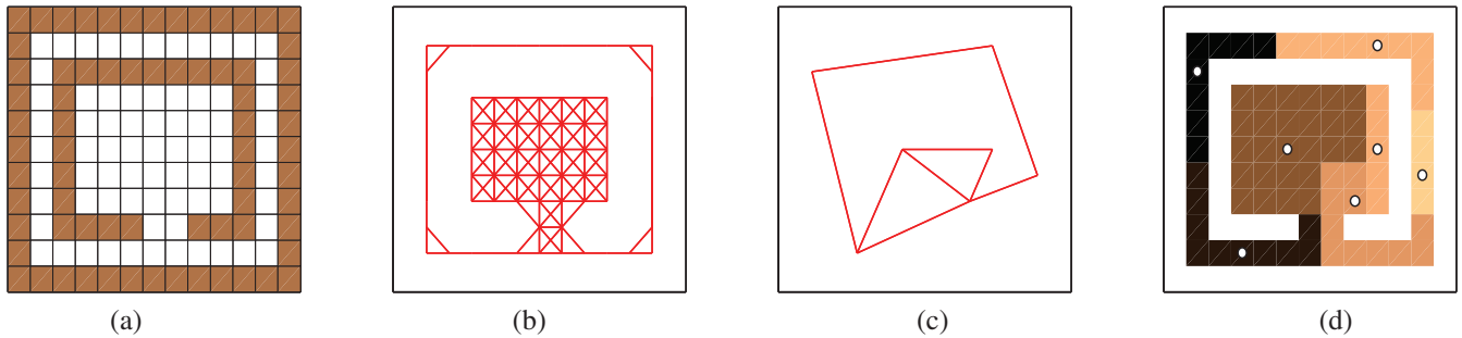
Figure 1: Clique-based abstraction employed by D LRTA*.
