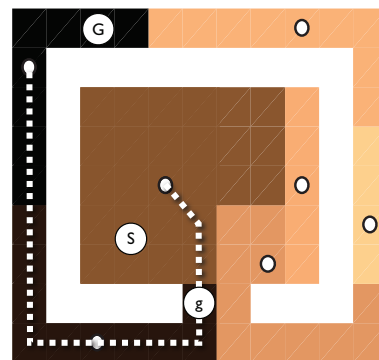
Figure 2: Subgoals as defined by D LRTA*. ‘S’ is the agent’s state, ‘G’ is the global goal, ‘g’ is the subgoal.
