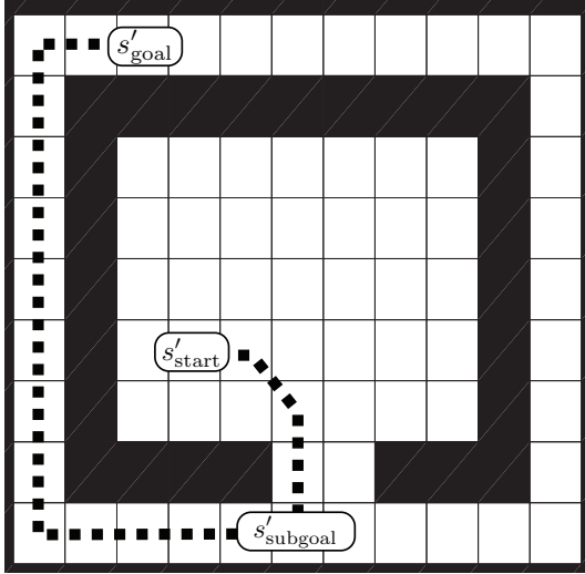
Figure 3: Subgoals as defined within kNN LRTA*.
