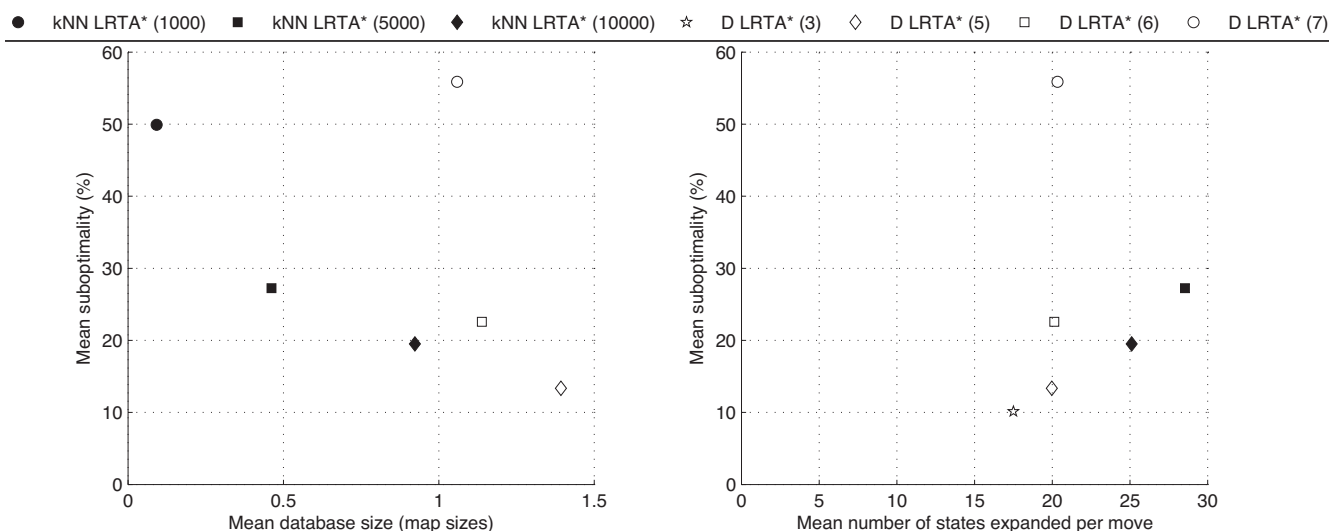
Figure 8: Suboptimality of paths as a function of database size and number of state expansions per move.
