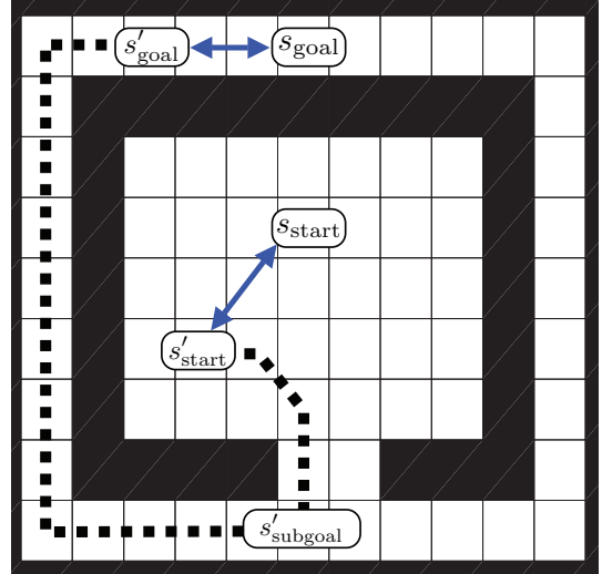
Figure 5: kNN LRTA* at runtime: finding the closest database entry. Double-ended arrows indicate heuristic distances between the agent’s situation (s_{start}, s_{goal}) and the closest database entry (s'_{start}, s'_{goal}, s'_{subgoal}) .
