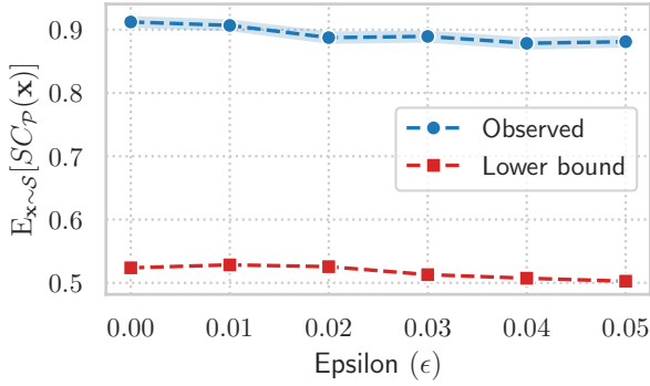
Figure 3: Observed versus worst-case expected self-consistency on the test set for varying values of \epsilon . While the lower bound becomes increasingly pessimistic as \epsilon grows, the observed average self-consistency remains high.
