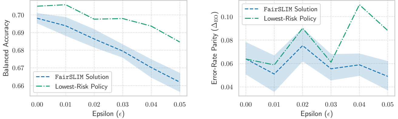
(a) Balanced accuracy of the best FairSLIM solution and the lowest-risk policy over the model pool \mathcal{P} for varying values of \epsilon .
