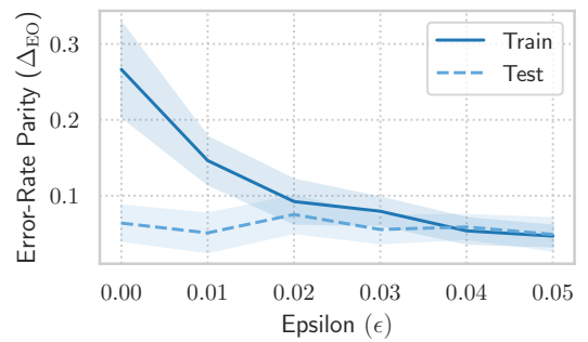
Figure 1: Error-rate parity ( \Delta_{\text{EO}} ) achieved by the least discriminatory model learned using FairSLIM on the train and test sets for varying values of \epsilon . A tolerance of \epsilon \leq .01 is sufficient to create a model pool with reduced error-rate disparities ( \leq 5\% ) on the test set.
