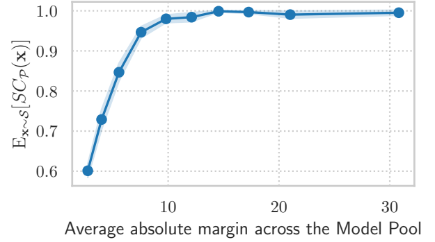
Figure 4: Expected self-consistency as a function of average absolute margin across the aggregated model pool \mathcal{P} for \epsilon \leq .01 . Predictive disagreement is concentrated among low-margin instances, while high-margin instances have almost perfectly consistent predictions.
