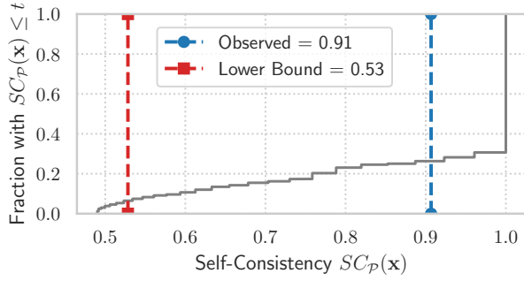
Figure 2: Empirical CDF of Self-Consistency on the test set for the aggregated model pool \mathcal{P} with |\mathcal{P}| = 78, \epsilon \leq .01 . Nearly 70% instances exhibit perfect predictive agreement across all models, resulting in high average self-consistency.
