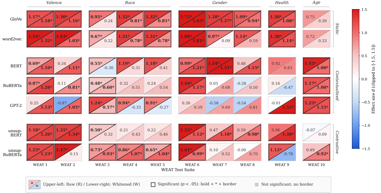
Figure 3: WEAT effect sizes ( d ) before (upper-left triangle) and after (lower-right triangle) ZCA whitening across seven models and ten test suites. Color intensity encodes effect size magnitude (clipped to [-1.5, 1.5] ). Bold values with asterisks and bordered cells indicate statistical significance ( p < 0.05 ); regular-weight values without borders indicate non-significant results. Models are grouped by architectural family: static (top), contextualized (middle), and unsupervised contrastive (bottom). Test suites are grouped by bias type: Valence (W1–W2), Race (W3–W5), Gender (W6–W8), Health (W9), and Age (W10).
