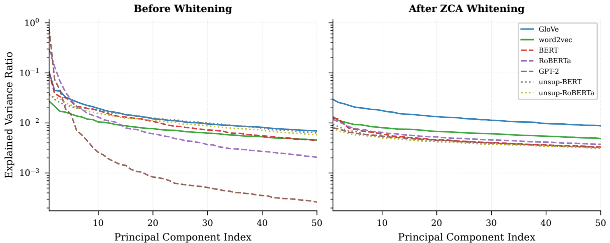
Figure 2: Explained variance ratio of the top 50 principal components (log scale) before (left) and after (right) ZCA whitening for all seven models. Left: Contextualized models (GPT-2, RoBERTa, BERT) show extreme variance concentration in the first few components, while static models (GloVe, word2vec) and contrastive models (unsup-BERT, unsup-RoBERTa) exhibit flatter distributions. Right: After whitening, all models converge to a near-uniform eigenvalue distribution.
