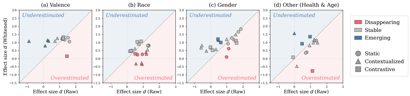
Figure 4: Scatter plots of WEAT effect sizes before (x-axis) and after (y-axis) ZCA whitening, separated by bias type: (a) Valence, (b) Race, (c) Gender, and (d) Other (Health & Age). The diagonal line represents no change; points above the line indicate increased effect sizes after whitening (underestimation in the raw space), and points below indicate decreased effect sizes (overestimation). Marker color denotes significance change: Disappearing (red), Stable (pink), and Emerging (blue). Marker shape denotes architectural family: circle (static), triangle (contextualized), and square (contrastive).
