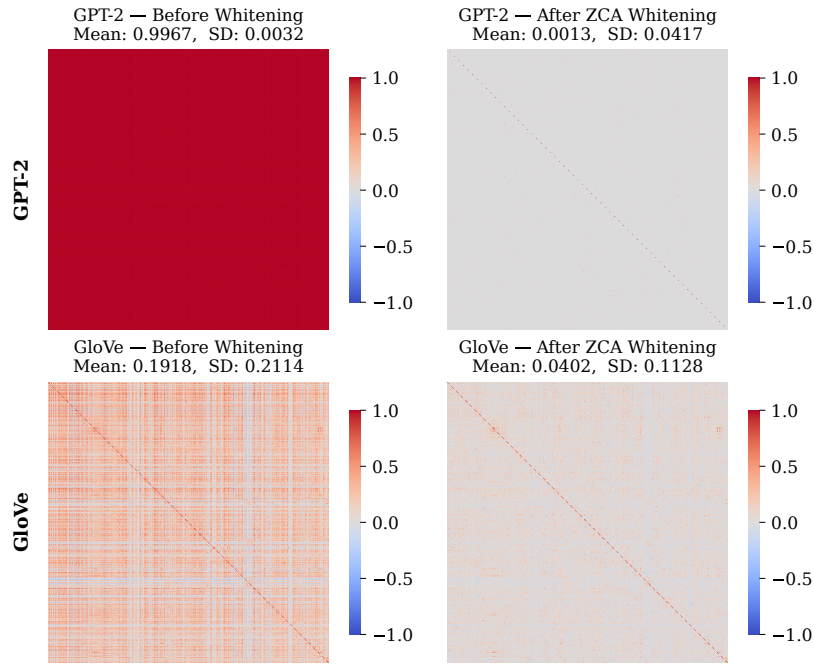
Figure 1: Pairwise cosine similarity matrices for 2,000 randomly sampled embedding vectors from WikiText-103 before (left column) and after (right column) ZCA whitening. Top: GPT-2, whose extreme anisotropy (mean cosine similarity = 0.997) renders the matrix a uniform red field. Bottom: GloVe (mean = 0.192), which exhibits moderate anisotropy before whitening. After calibration, both models converge to near-zero mean similarity with meaningful pairwise variation restored.
