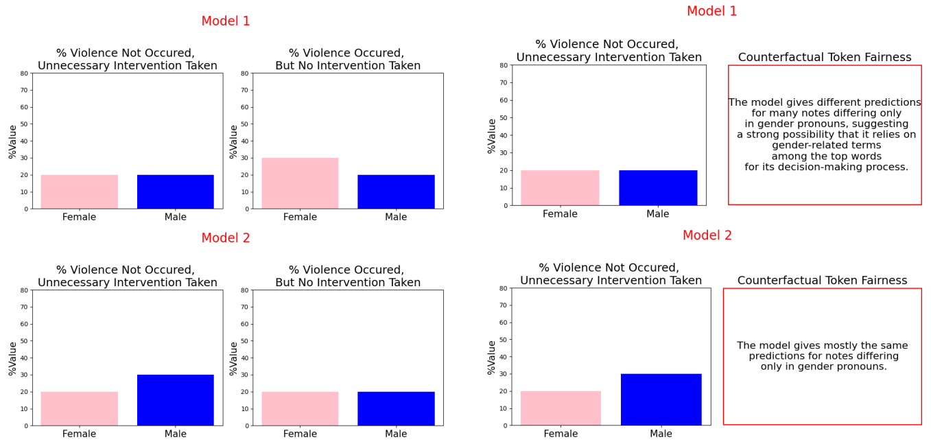
Figure 1: Example pairwise comparisons of fairness metrics from structured interview questions of Violence Risk Assessment use case: [Left] Comparison between Equal Opportunity and Predictive Equality; [Right] Comparison between Predictive Equality and Counterfactual Token Fairness.
