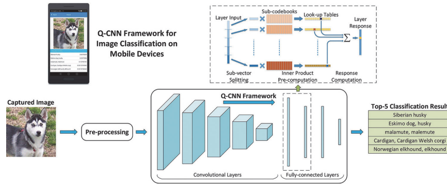
Figure 2: The workflow of the image classification process on mobile devices, based on our Q-CNN framework.
