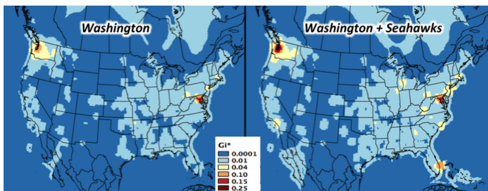
Figure 2: Left: Local G_{i^*} values for Washington . Right: interpolated G_{i^*} values for Washington + Seahawks .
