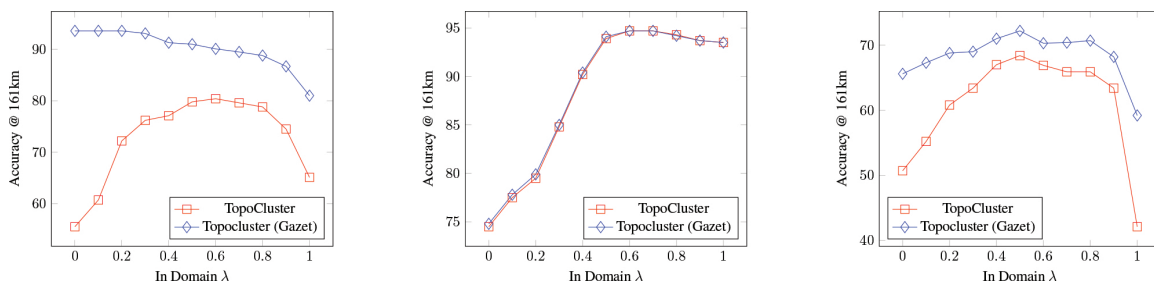
Figure 3: Domain adaptation: optimizing \lambda for each corpus. Left: TR-CoNLL, Middle: CWar, Right: LGL.
