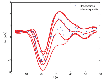
(a) Variational Bayesian.
