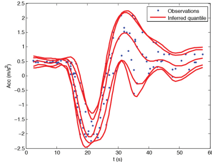
(b) Expectation Propagation
