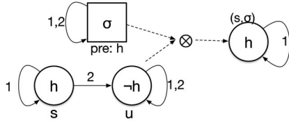
Figure 2: Lost of seriality
