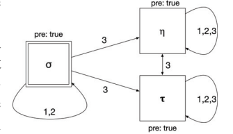
Figure 11: (\Sigma_{flip}^2, \{\sigma\})
