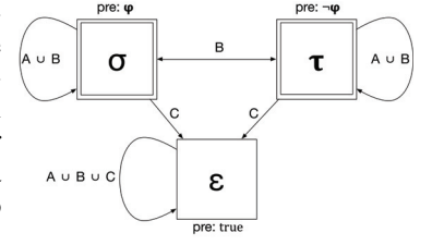
Figure 7: \Sigma^{Sensing}(A; B; \varphi)
