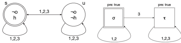
Figure 8: (\mathcal{M}_0, s) (left) and (\Sigma_{flip}, \{\sigma\}) (right)
