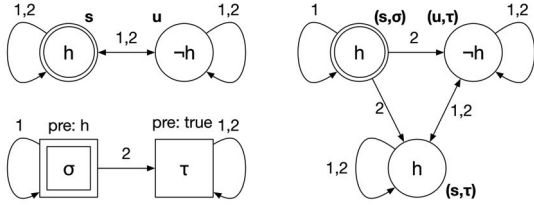
Figure 1: Knowledge as true belief
