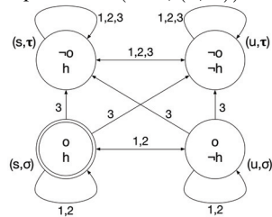
Figure 9: (\mathcal{M}_1, (s, \sigma))
