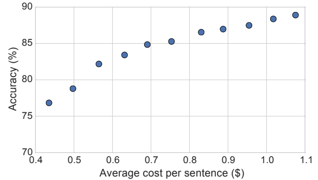
Figure 3: Budgeteer's accuracy vs cost per sentence.
