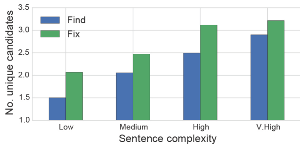
Figure 2: The average number of unique fix and find candidates identified by Budgeteer per sentence complexity.
