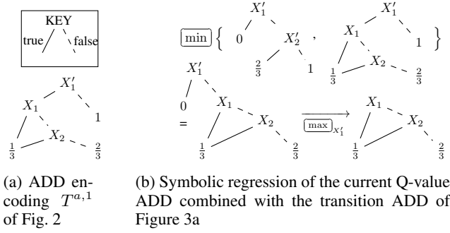
Figure 3: Algebraic Decision Diagrams for PPUDD
