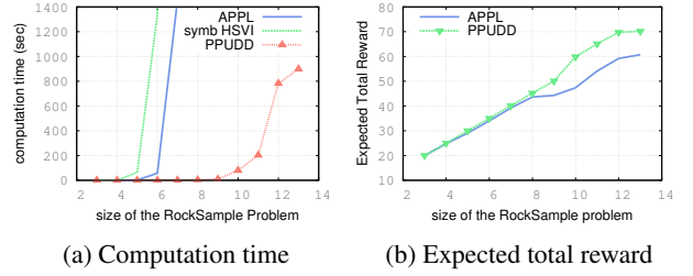
Figure 6: PPUDD vs. APPL and symb HSVI (RS)
