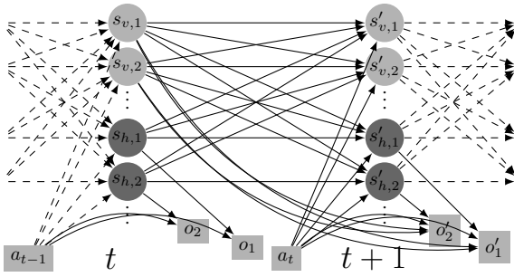
Figure 4: DBN of a factored belief-independent \pi -MOMDP
