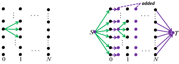
Figure 3: Left: Original Grid; Right: Constructed Network in which all the edges have capacity 1. Only the added purple edges have non-zero weights, with the weight of such an edge equaling the sum of all the target weights covered by the corresponding grid point.
