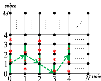
Figure 1: Discretized Grid.
