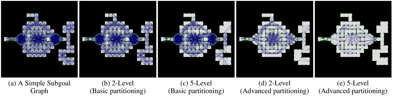
Figure 3: N-Level Subgoal Graphs constructed using basic partitioning and advanced partitioning that is allowed to add h-reachable edges. (Only the highest level vertices and the edges between them are shown.)
