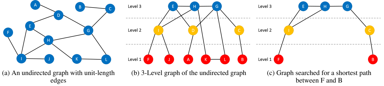
Figure 2: Idea behind N-Level graphs.
