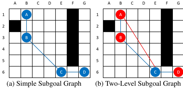
Figure 1: Simple and Two-Level Subgoal Graphs (local subgoals are shown in red).
