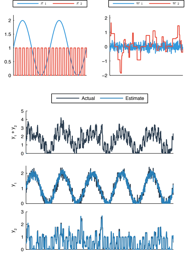
Figure 1: Synthetic data generation process starting with two underlying signals (top left), corrupted by different noise models (top right), summed to give the observed input (row 2) and disaggregated (rows 3 and 4).
